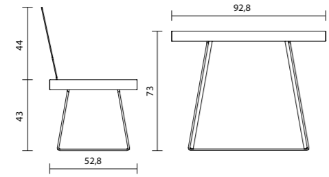
Bank bench banc Tisch table table
